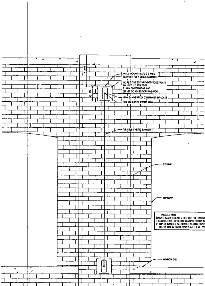
WALL ELEVATION SCALE 3/4 1-0
