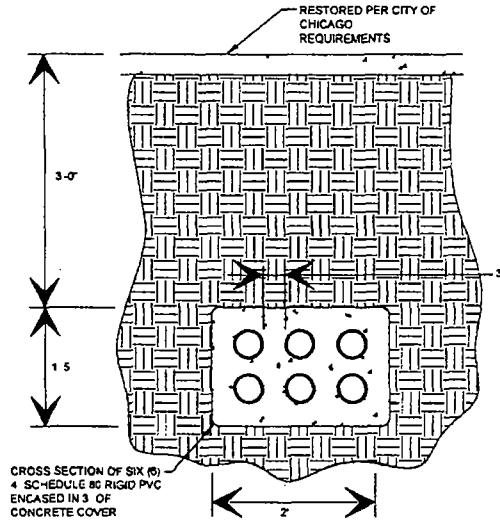
1 DUCT BANK SECTION
