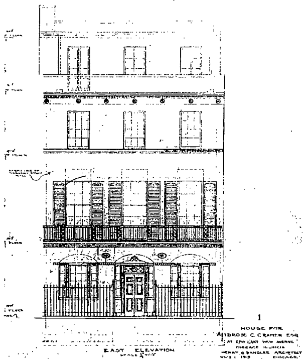
Image 42: Front elevation plan for 2710 North Lakeview Avenue for Cramer
