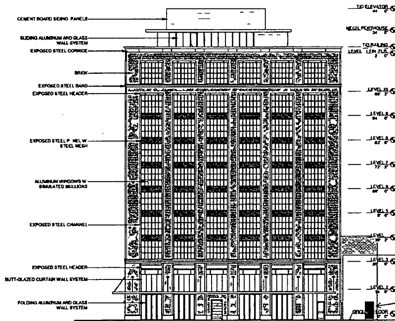
W Randolph/South Elevation
