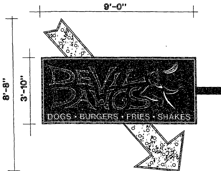
DETAIL OF DOUBLE TUBE NEON IN LETTER
