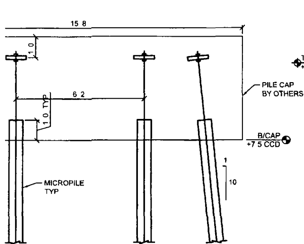
3 SECTION Scale 3/8" = 1'-0"
