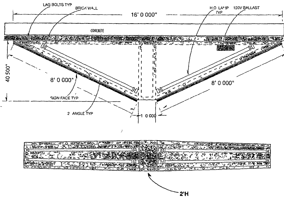
A SINGLE FACE WALL SIGN Scale 1/2"=1'
