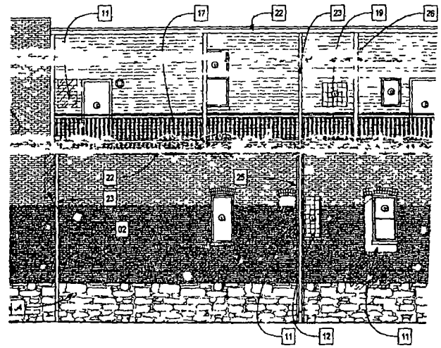
4 NORTH ELEVATION SCALE 1/8" = 1'-0"
