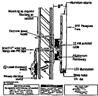
Front Lit Channel Letter on Raceway SECTION DETAIL
