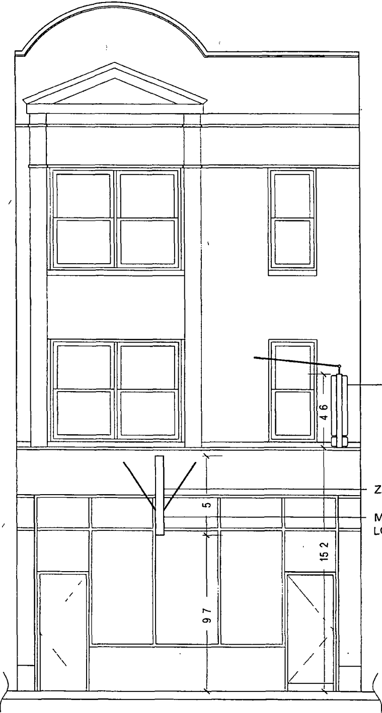
FRONT (NORTH) ELEVATION SCALE 3/16 = 1.0
