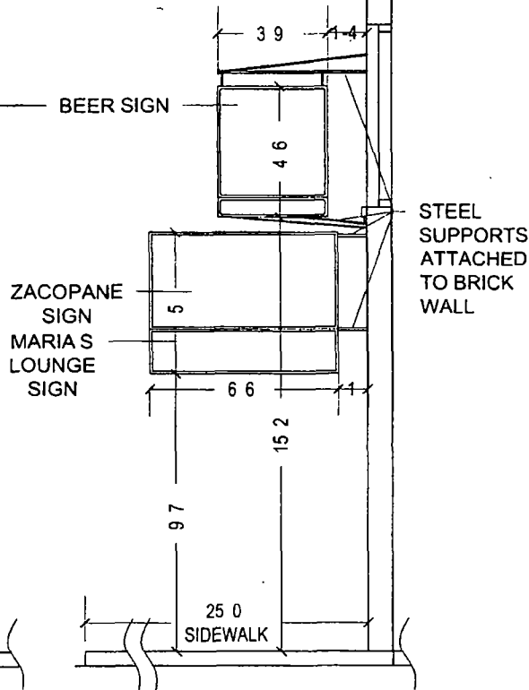
SECTION/ ELEVATION SCALE 3/16 = 1.0
