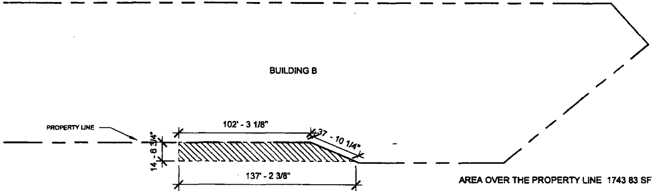
1 BUILDING B AREA SK-22 1" = 50'-0"
