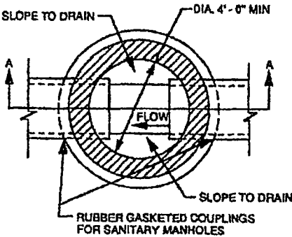
SECTIONAL PLAN
