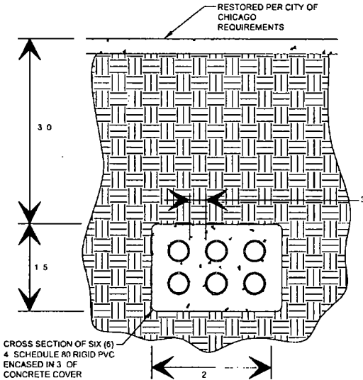
① DUCT BANK SECTION
