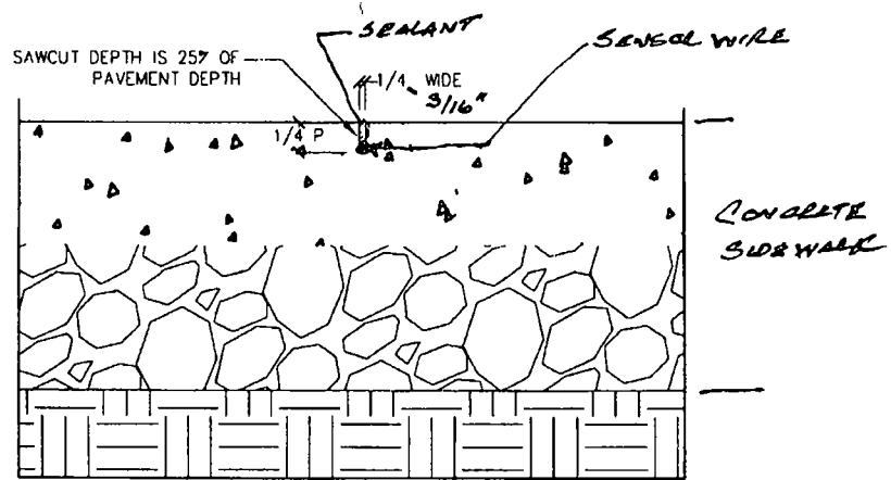
TRAFFIC SENSOR LOOP DETAIL SAWCUT IN SIDEWALK
