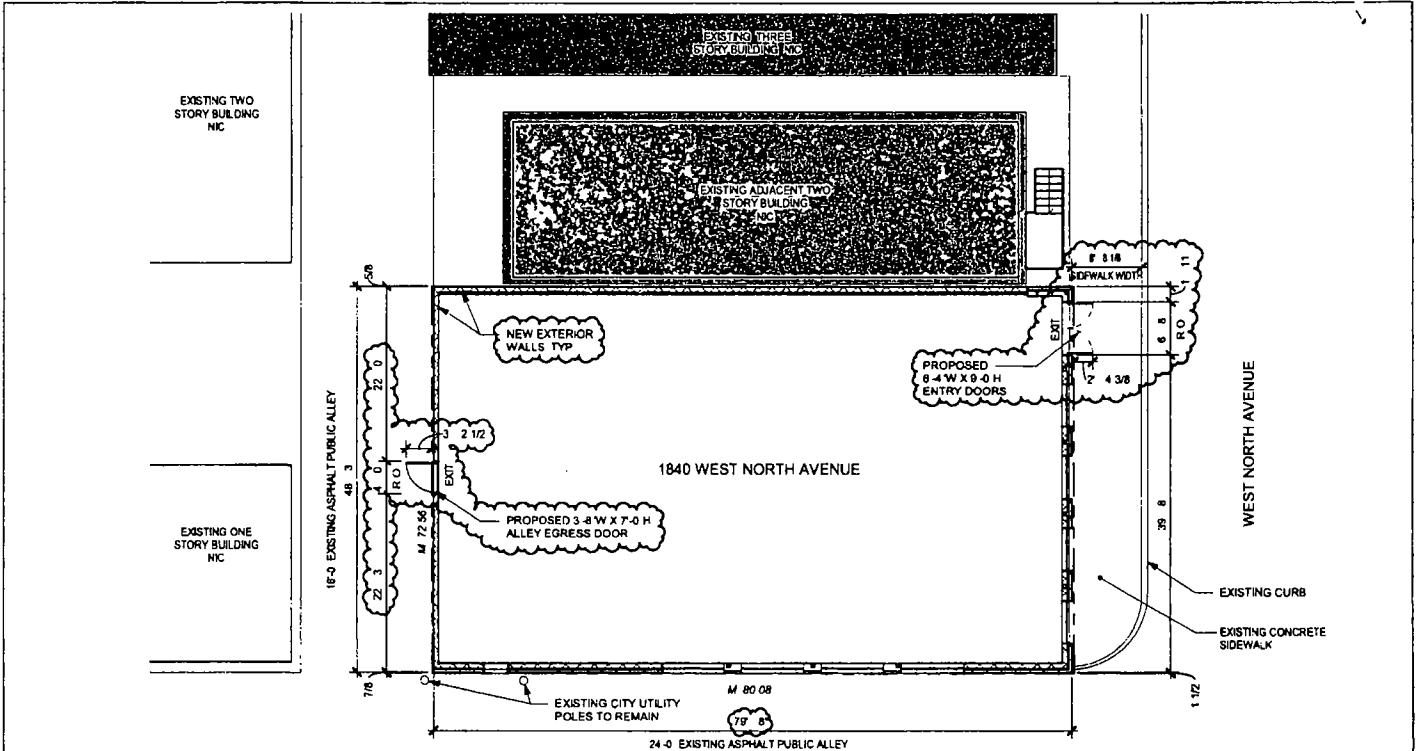
1 ARCHITECTURAL SITE PLAN PWA-01 SCALE 3/32 = 1'-0"
