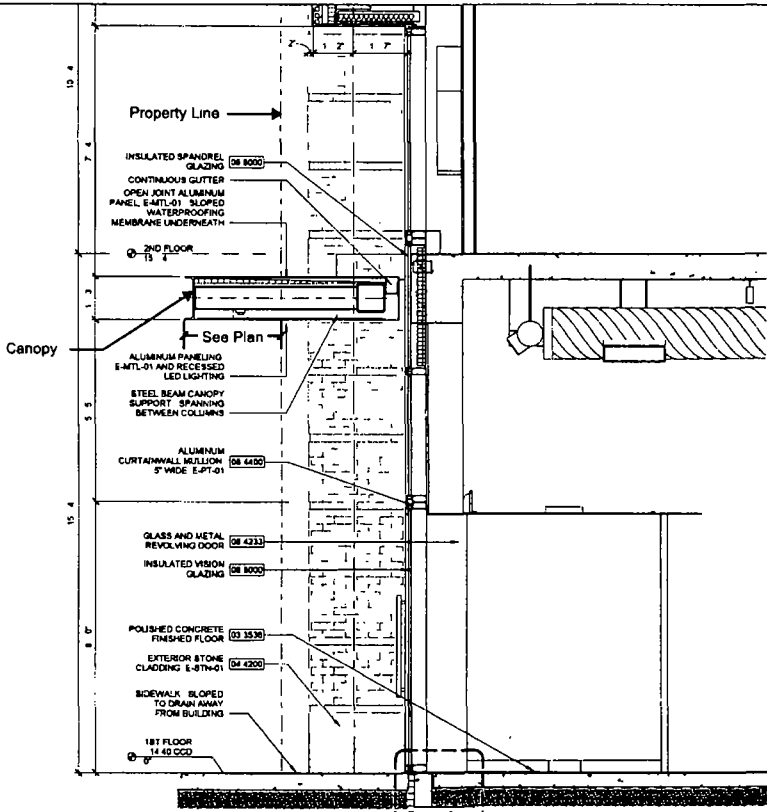
CANOPY SECTION NTS
