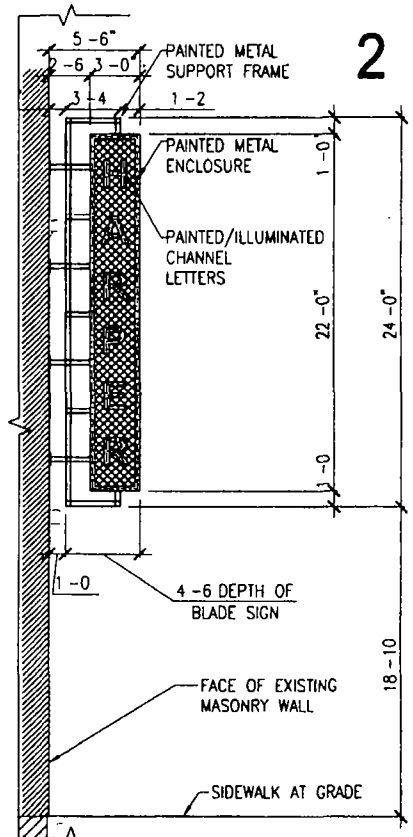
2 SECT THRU EAST WALL SCALE 1/2" = 1'-0"
