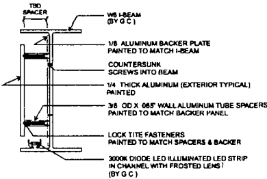
I-BEAM BAND OF LETTERS DETAIL SCALE 3/16"
