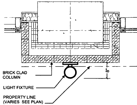
COLUMN PLAN DETAIL AT LIGHT FIXTURE NTS
