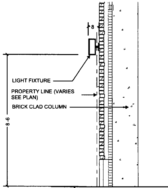
COLUMN SECTION AT LIGHT FIXTURE NTS
