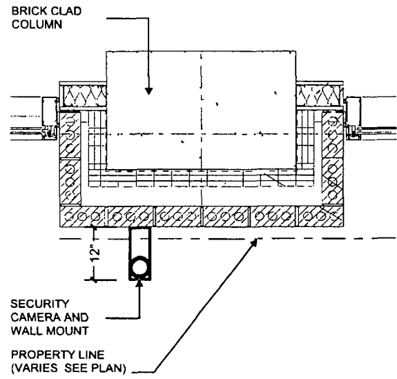
COLUMN PLAN DETAIL AT SECURITY CAMERA NTS
