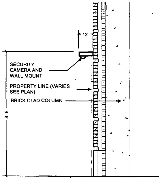
COLUMN SECTION AT SECURITY CAMERA NTS
