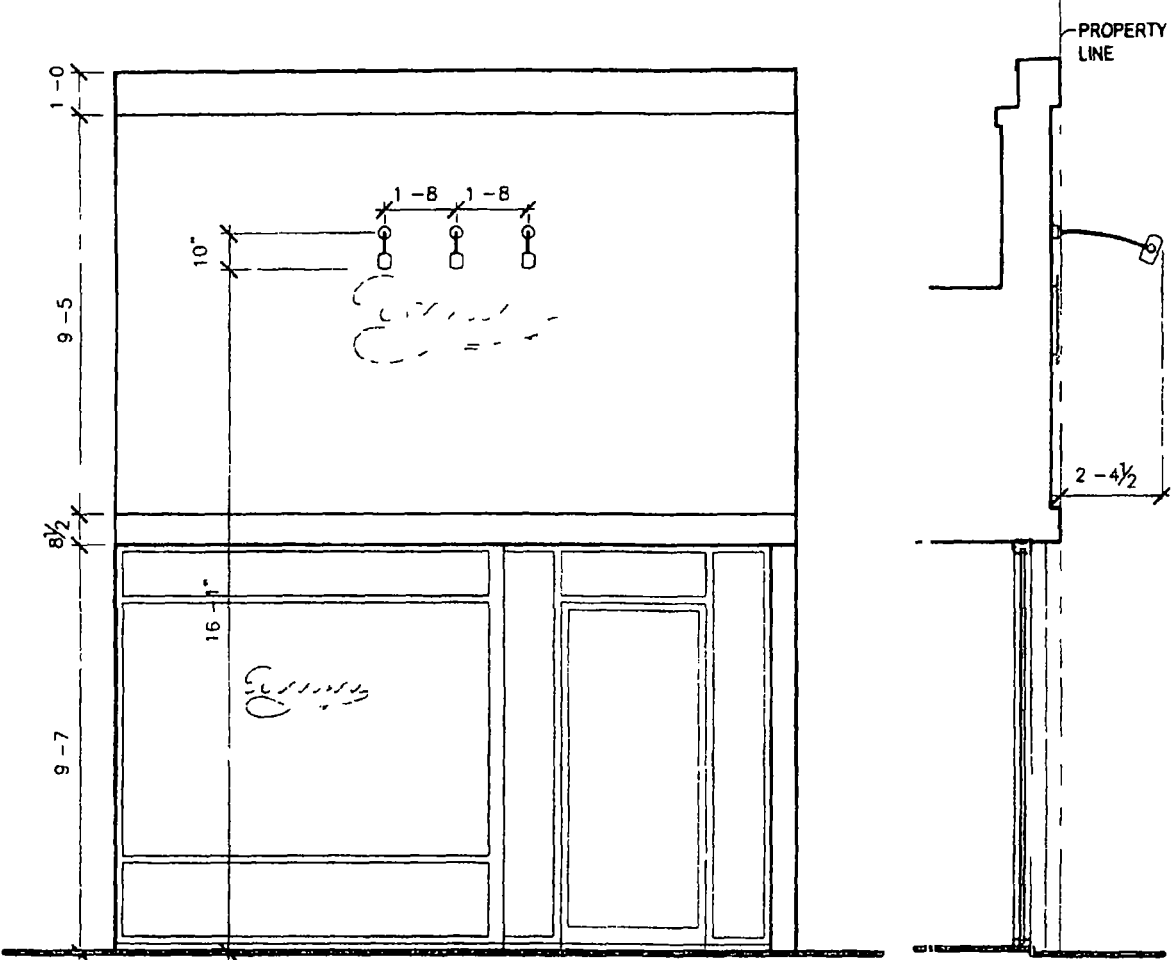
STOREFRONT ELEVATION 1/4" = 1'-0"
