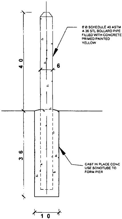
2 BOLLARD DETAIL SCALE 1/2" = 1'-0"
