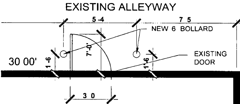
3 ENLARGED PLAN OF THE REAR EXIT SCALE 1/4" = 1'-0"
