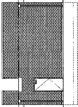
WEST ELEVATION SCALE: 1/4" = 1'-0"
