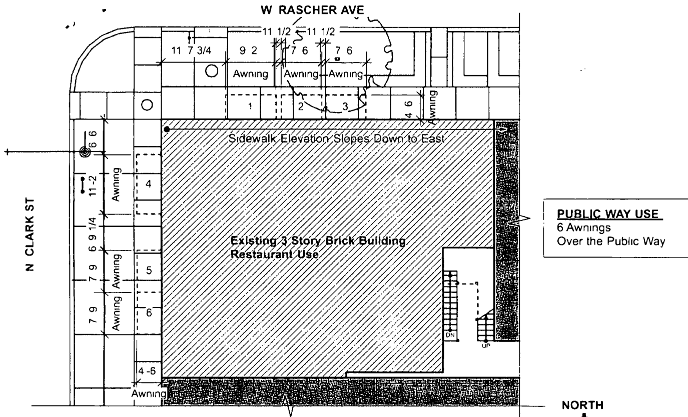
SITE PLAN SCALE 1/16" = 1'-0"
