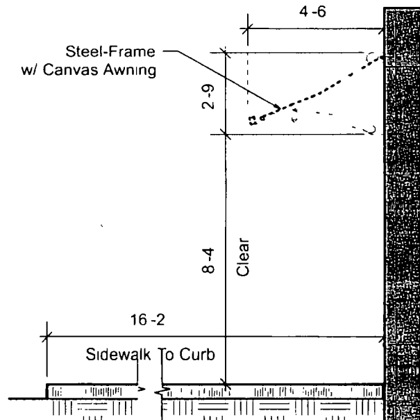
CLARK ST SECTION (4, 5, & 6) SCALE 1/4" = 1'-0"
