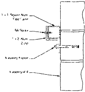
Mounting Detail
