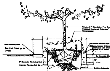
PROPOSED TREE WITH NEW PLANTER SECTION DETAIL NTS
