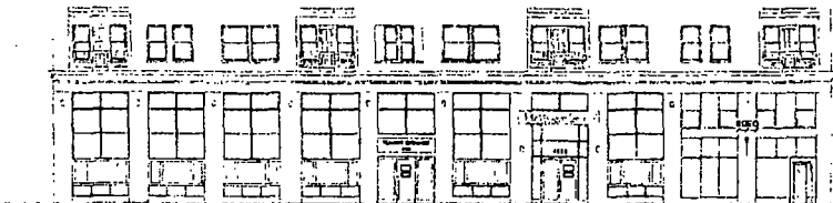
WEST ELEVATION
