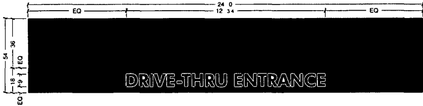
AWNING SIGN 8 SCALE 3/8" = 1' 0" QTY 1
