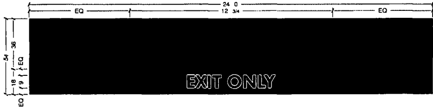
AWNING SIGN 10 SCALE 3/8" = 1' 0" QTY 1
