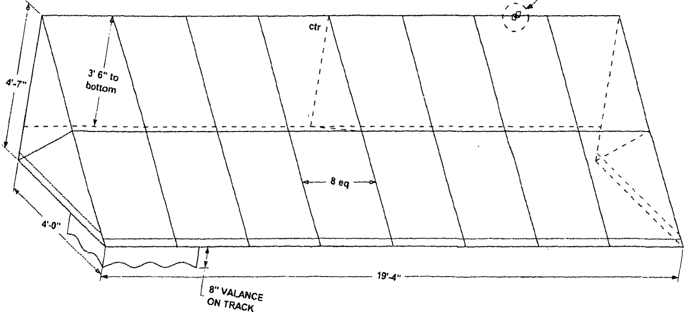
ISOMETRIC VIEW S103
