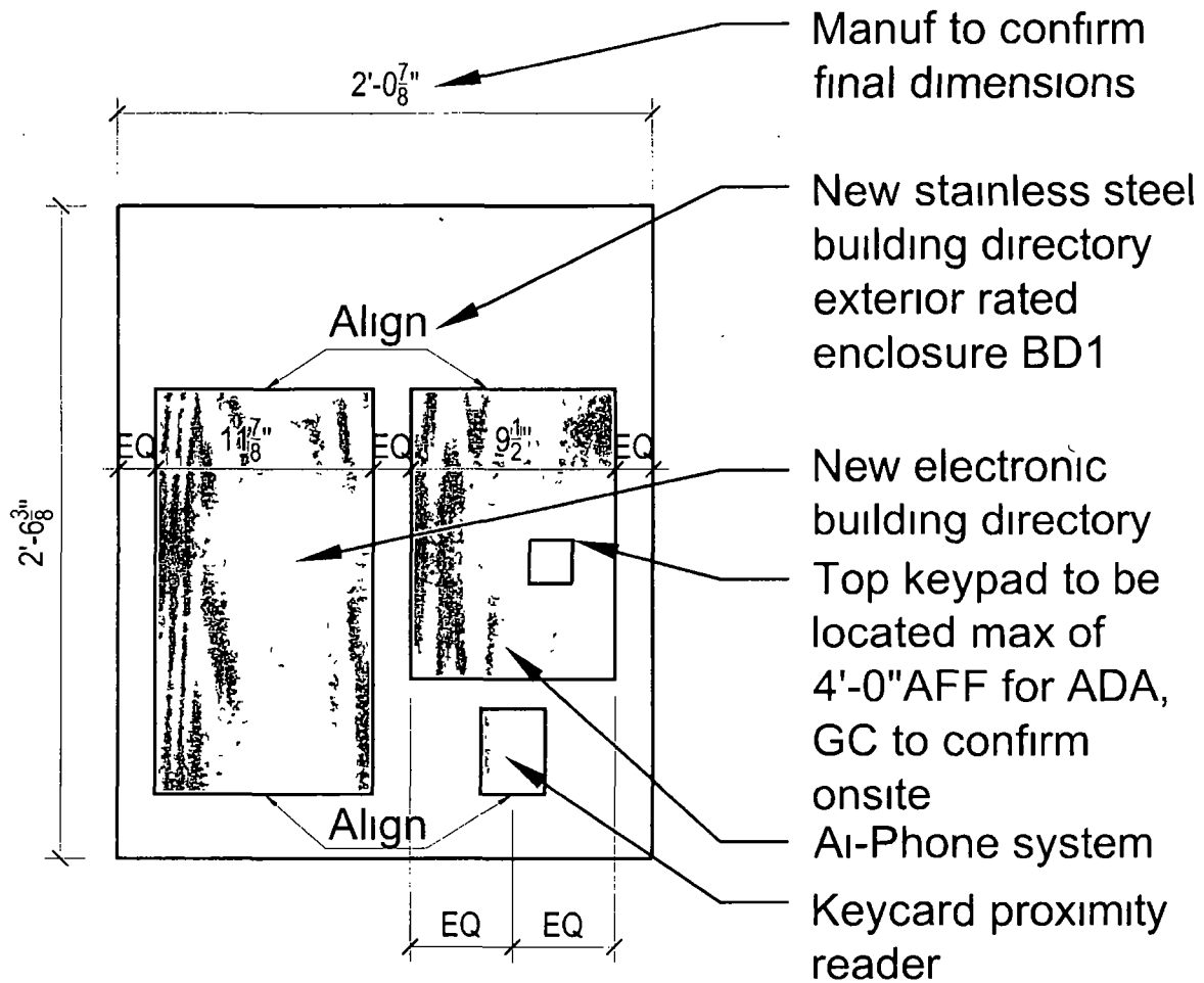
6 Elevation Building Diretory BD1 Scale 1/4"=1'-0"
