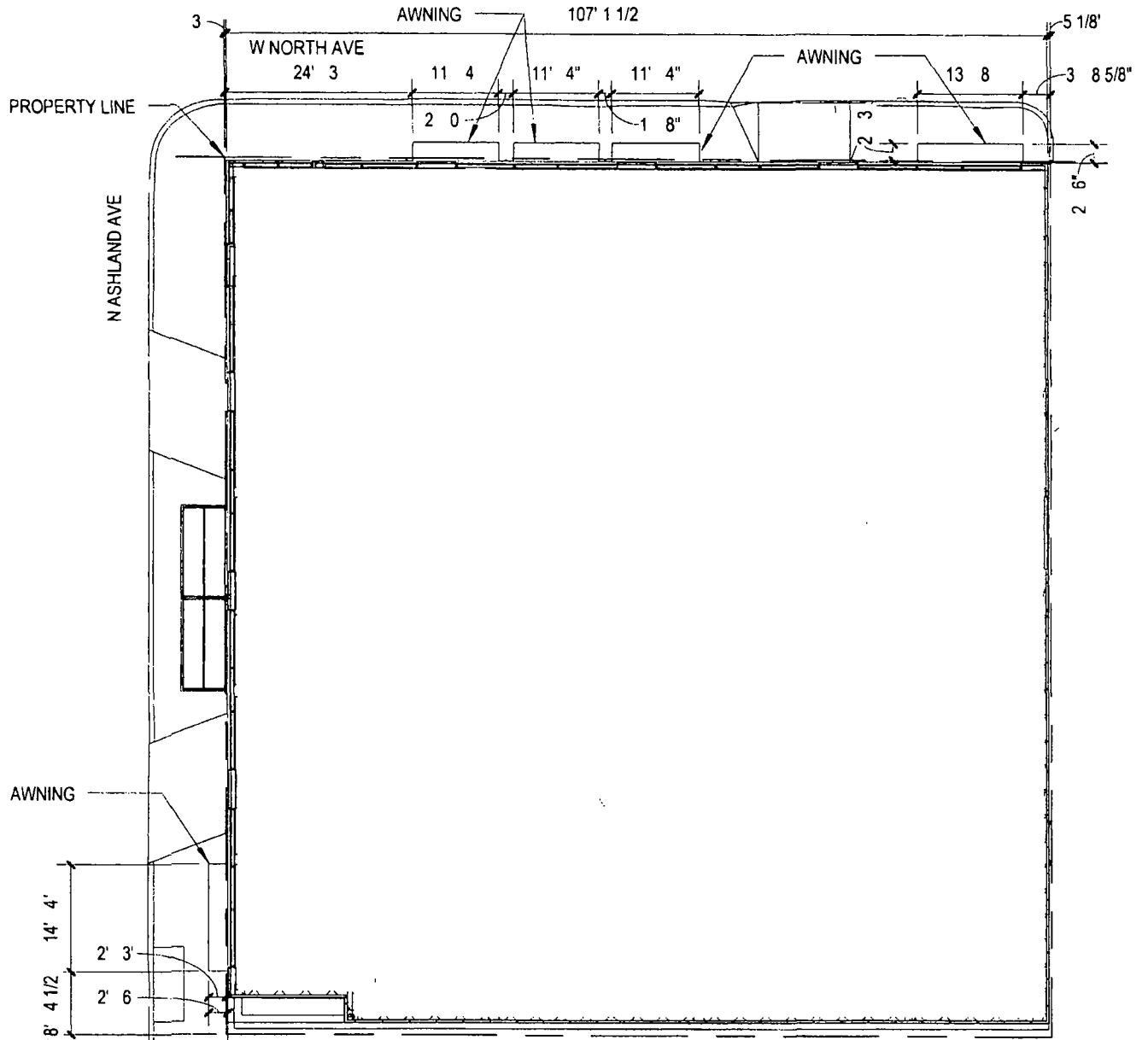
PLAN DRAWING
