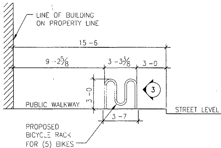
2 FRONT ELEVATION
