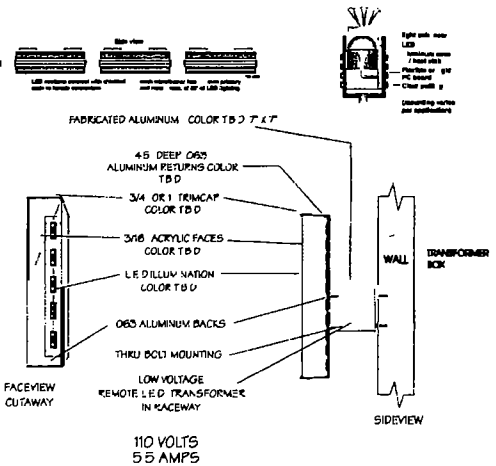
TYPICAL LED ILLUMINATED CHANNEL LETTER MOUNTED TO WIREWAY
