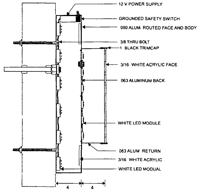
Typical U.L. LED Illuminated Routed Alum Cabinet with Channel Letters
