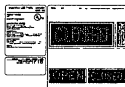
B3 OPEN/CLOSED LED PANEL DETAIL SCALE: 1/8" = 1'-0"
