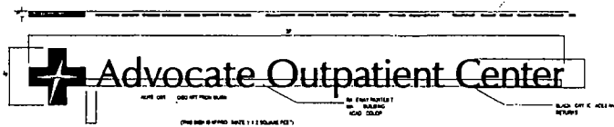
B1 NORTH ELEVATION BUILDING MOUNTED LOGO LOCATION 1 SIGN TYPE E3 SCALE: 1/8" = 1'-0"
