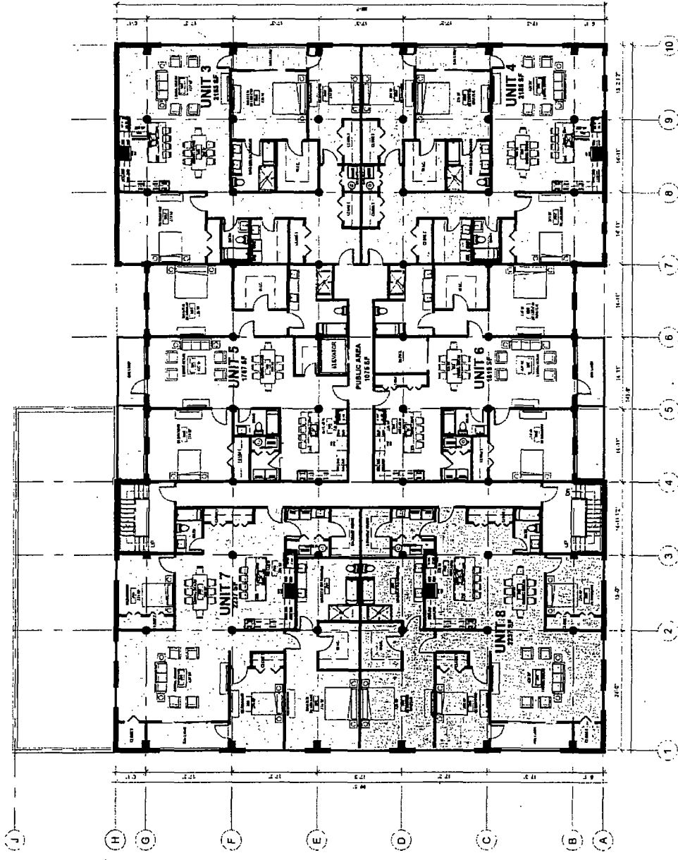
SECOND FLOOR SCALE: 1/16" = 1'-0"
