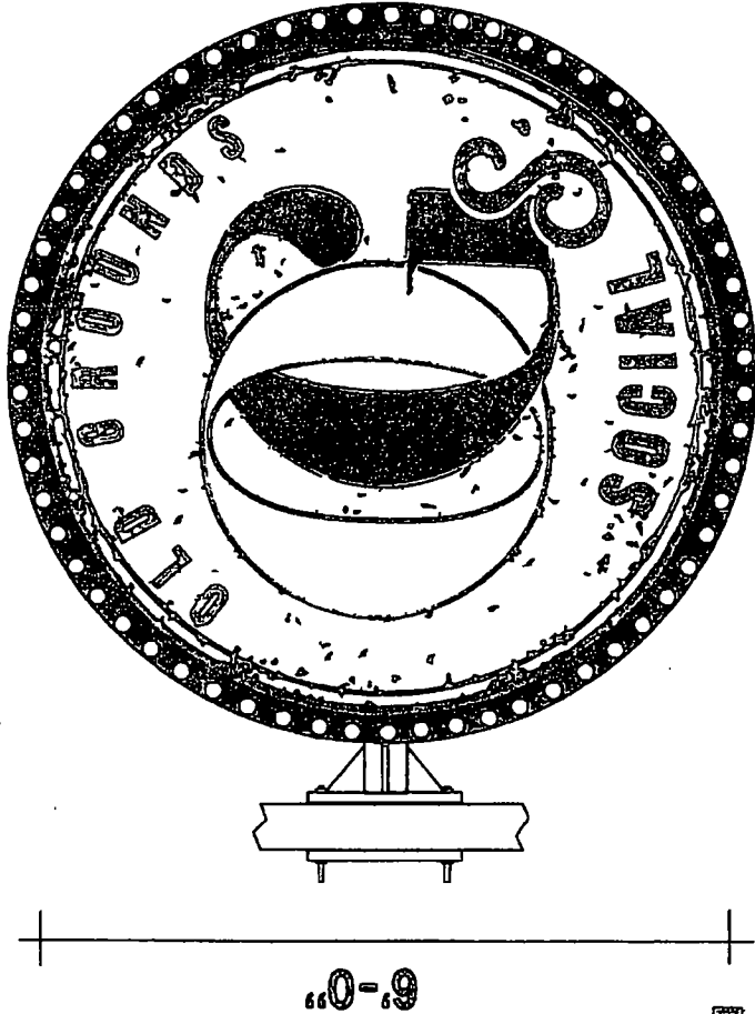
6'x6' PROJECTING SIGN WITH LEXAN FACE CLEAR 11 WATT BULBS ON BLACK BORDER
