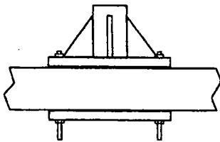
DETAIL OF BEAM MOUNT 4" STEEL TUBE/GUSSETS WELDED TO .5" STEEL PLATE/BOLTED TO BACKING PLATE WITH .5" GALV BOLT
