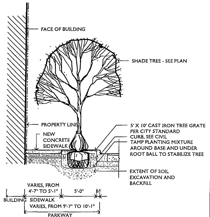
2 TYPICAL SECTION AT WEST ILLINOIS STREET
