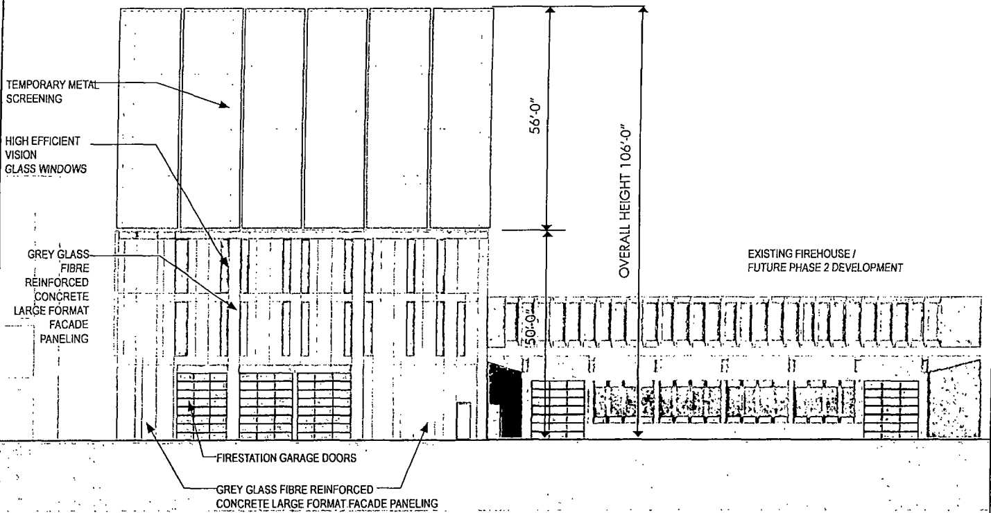
PHASE 1 FIREHOUSE - SOUTH ELEVATION SCALE 1" = 30'-0"
