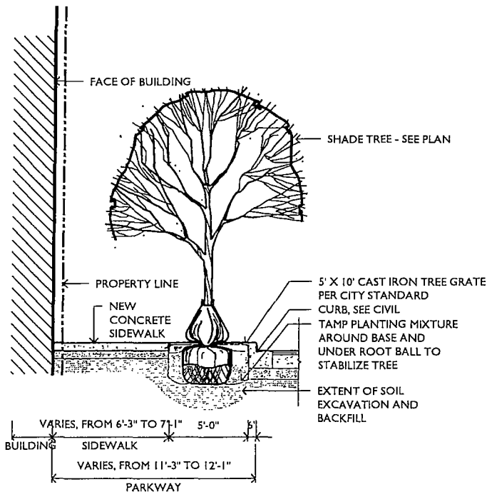
1 TYPICAL SECTION AT NORTH DEARBORN STREET
