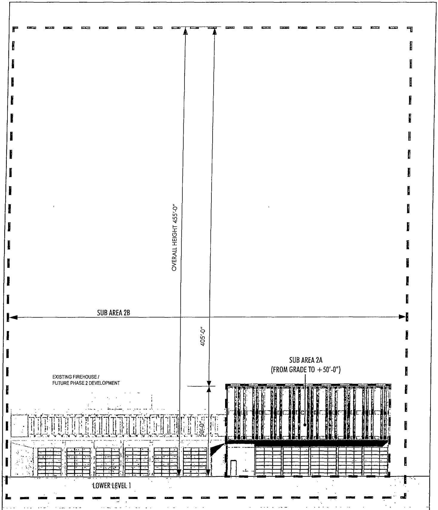
NORTH ELEVATION SUB AREA 2A/2B SEPARATION SCALE 1"=30'-0"
