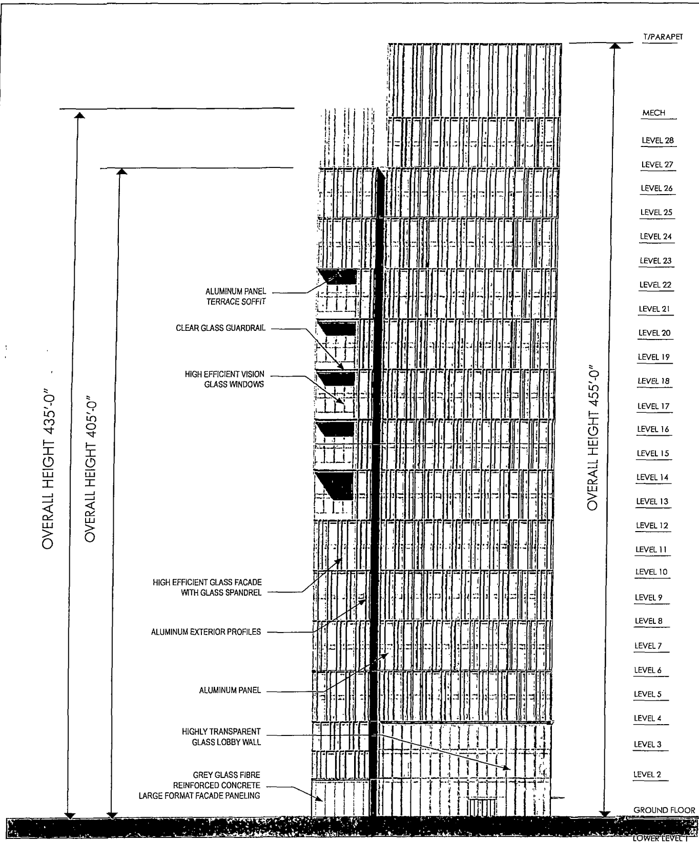
PHASE 2 EAST ELEVATION SCALE 1"=50'-0"
