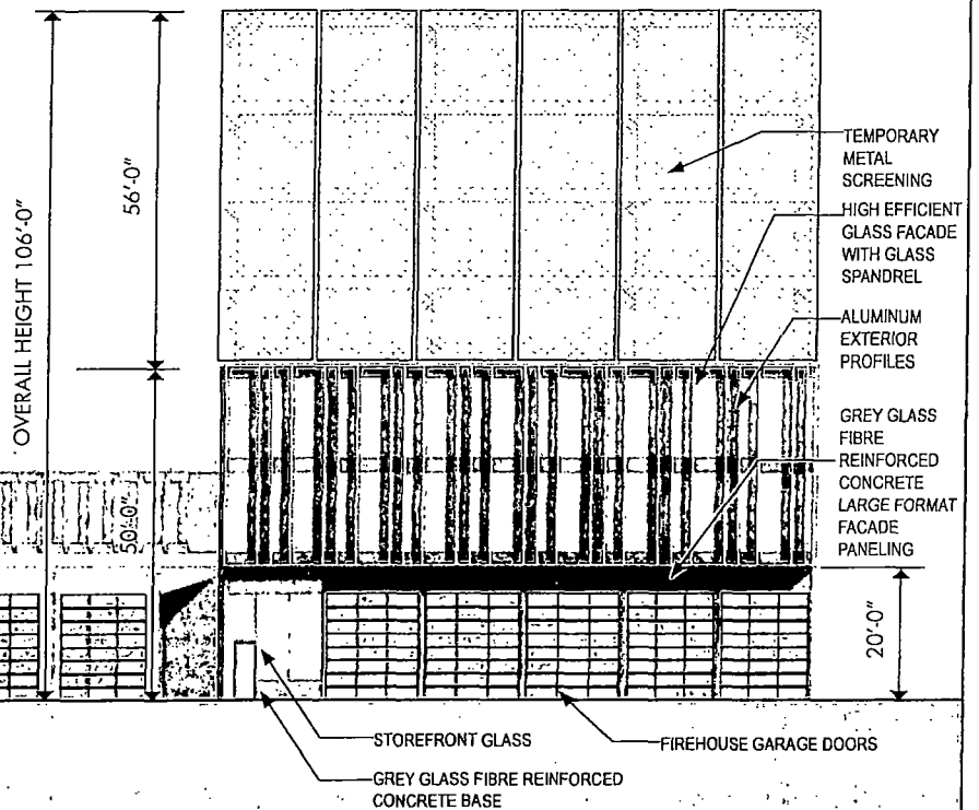
PHASE 1 FIREHOUSE - NORTH ELEVATION SCALE 1"=30'-0"
