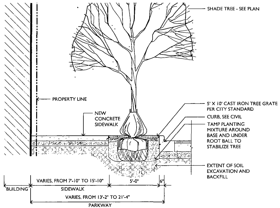
1 TYPICAL PARKWAY SECTION @ SOUTH CLINTON STREET AND SOUTH CANAL STREET
