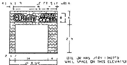
SOUTH ELEVATION FACING PARKING LOT
