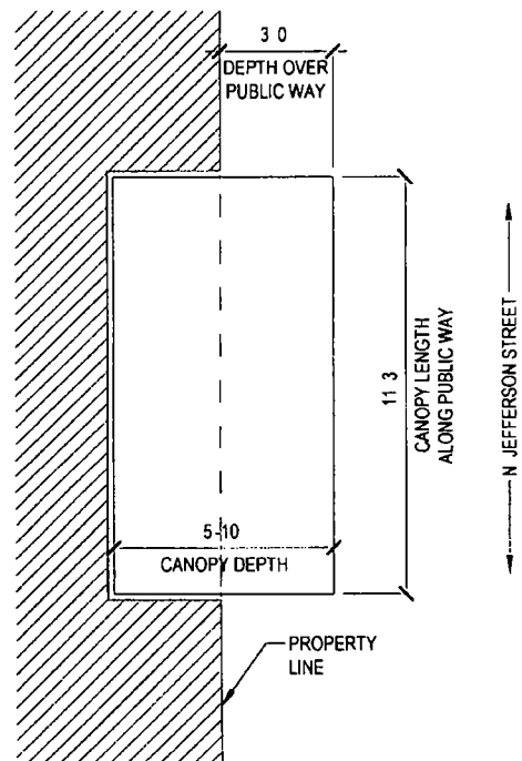
1 PLAN Scale 1/4" = 1'-0"
