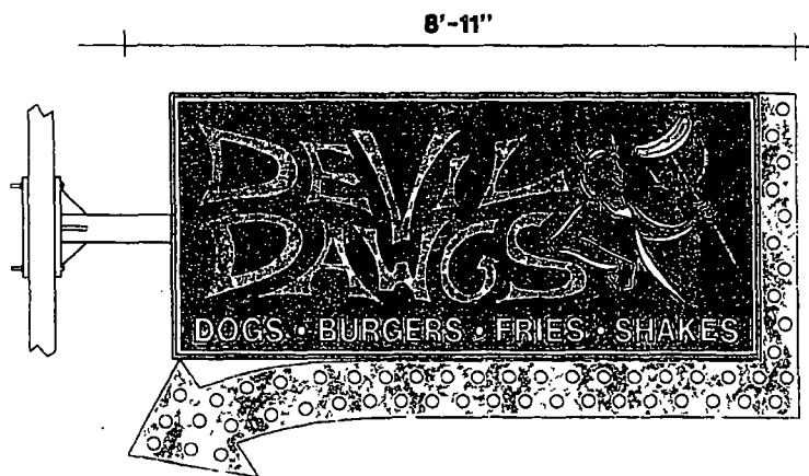
DOUBLE FACE PROJECTING SIGN
