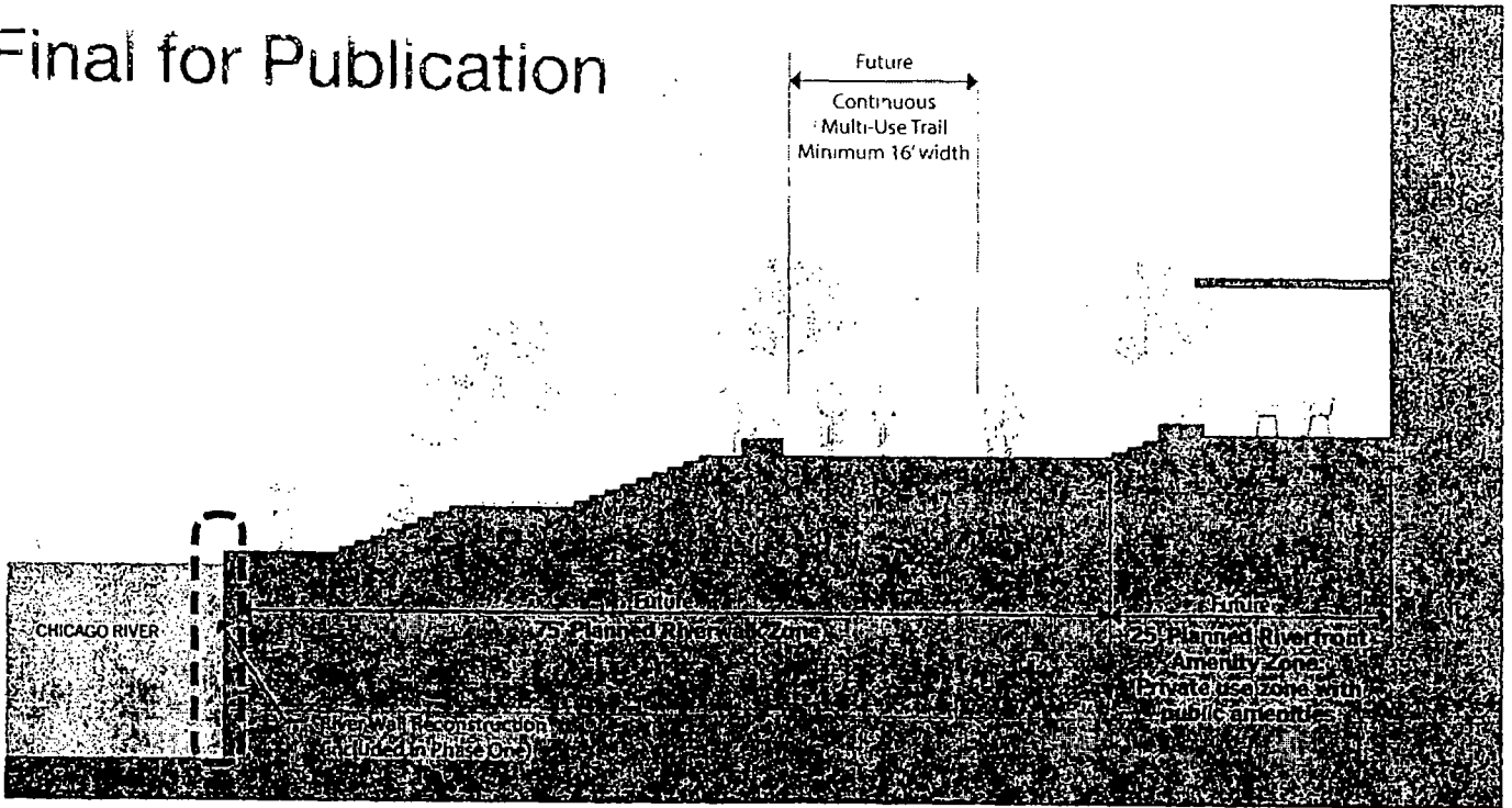
River Wall Section
