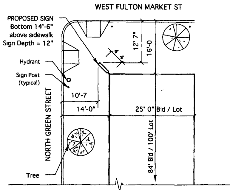
SITE PLAN
