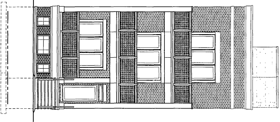
● B FRONT ELEVATION
