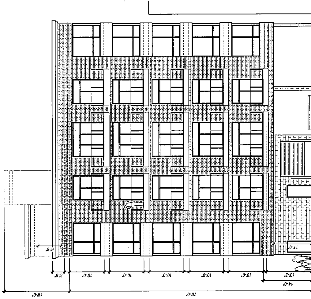
2 NORTH ELEVATION \frac{3}{32}" = 1'-0"
