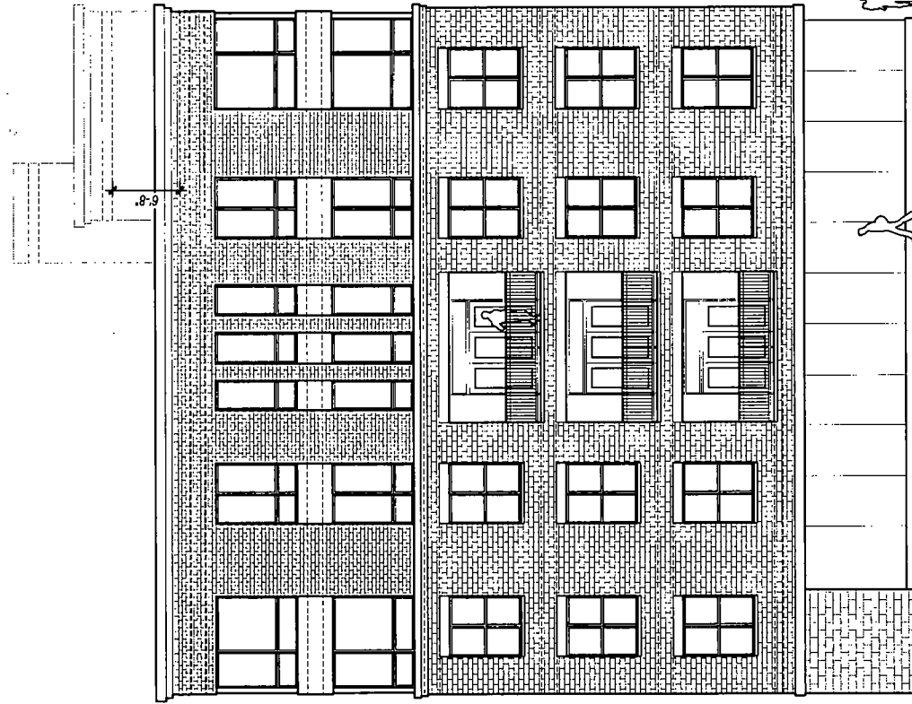
1 SOUTH ELEVATION \frac{3}{32}" = 1'-0"
