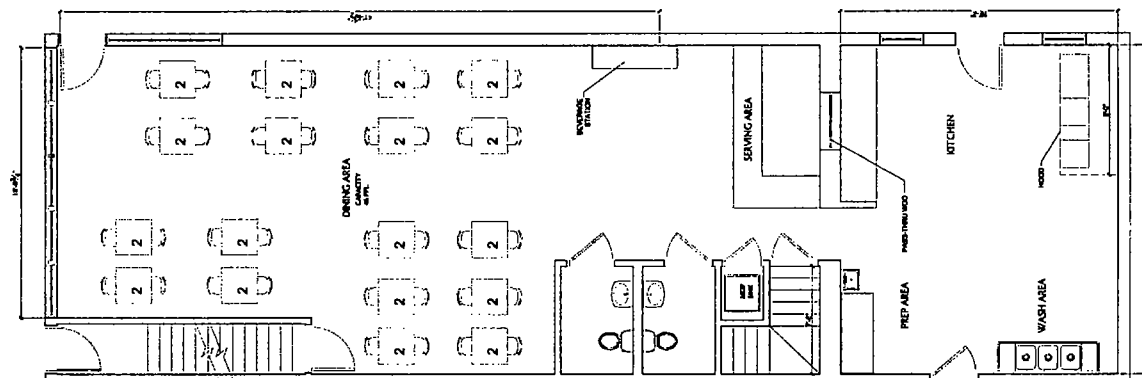
SCALE: 1/4" = 1'-0" FIRST FLOOR PLAN: DEMOLITION
