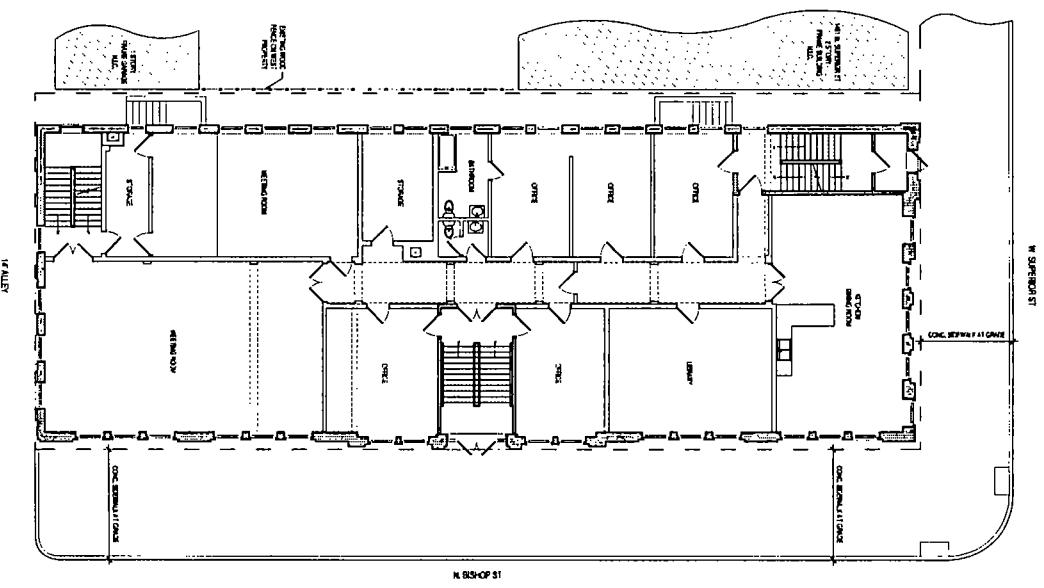
2 EXISTING FIRST FLOOR PLAN 15'-0" x 12'-0"
