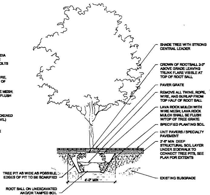
2 SHADE TREE IN PAVER GRATE SECTION 1/8"=1'-0"
