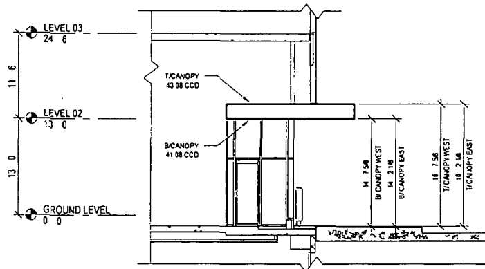
NORTH/SOUTH SECTION
