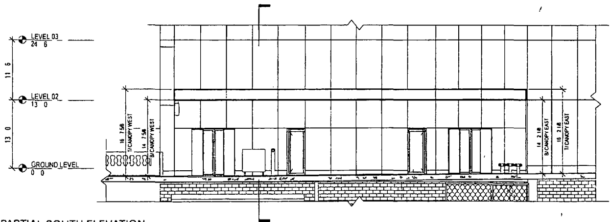
PARTIAL SOUTH ELEVATION
